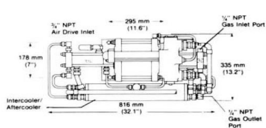
Double acting, two stage, single air head 8AGT-30/60
