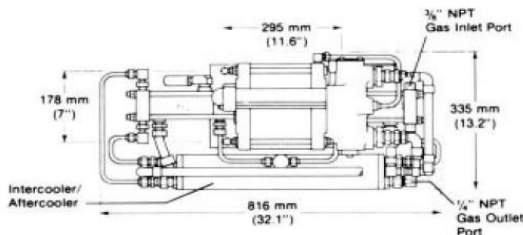
Double acting, two stage, single air head 8AGT-14/60
