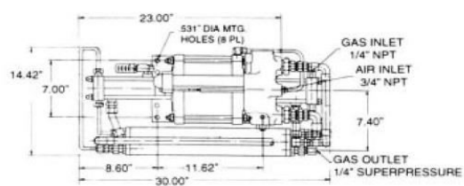
Double acting, two stage, single air head 8AGT-60/150
