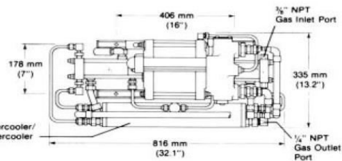
Double acting, two stage, single air head 8AGT-14/30
