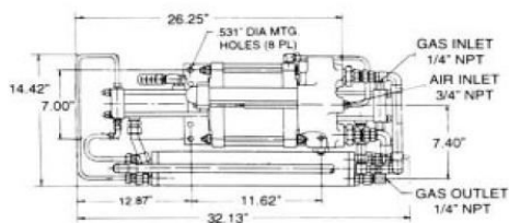
Double acting, two stage, single air head 8AGT-30/150
