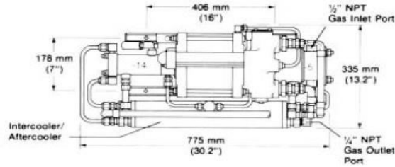
Double acting, two stage, single air head 8AGT-5/14
