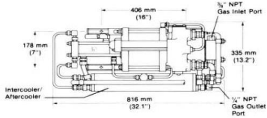
Double acting, two stage, single air head 8AGT-5/30
